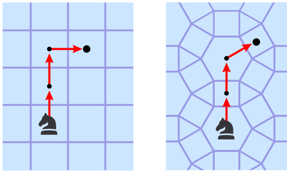
Figure 3: Relative knight move \{0, 0, 1\} on the square grid (left) and the semi-regular 3.4.6.4 grid (right).
