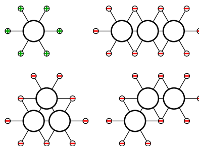
Figure 7: Patterns for a “form groups of 3” strategy.
